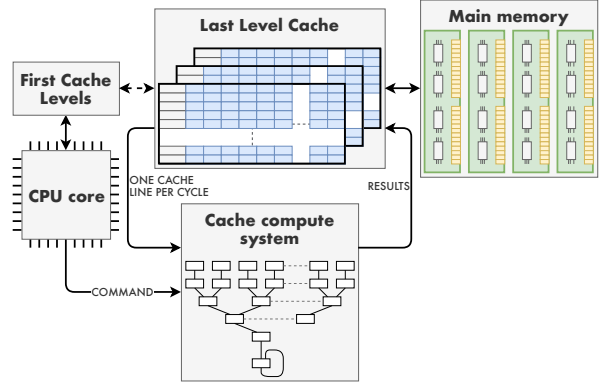
Fig. 2 Block diagram of the proposed system integrating a processing core with the CCS.
