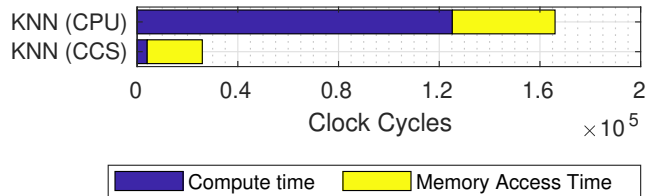
Fig. 9 Performance results regarding the distance computation phase of the kNN algorithm, showing the time dedicated to accessing the memory and the actual computation time.
