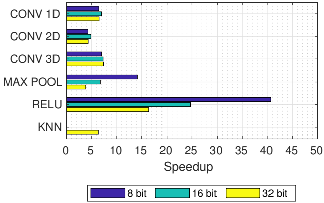
Fig. 10 Speedup allowed by executing six kernels using the CCS.
