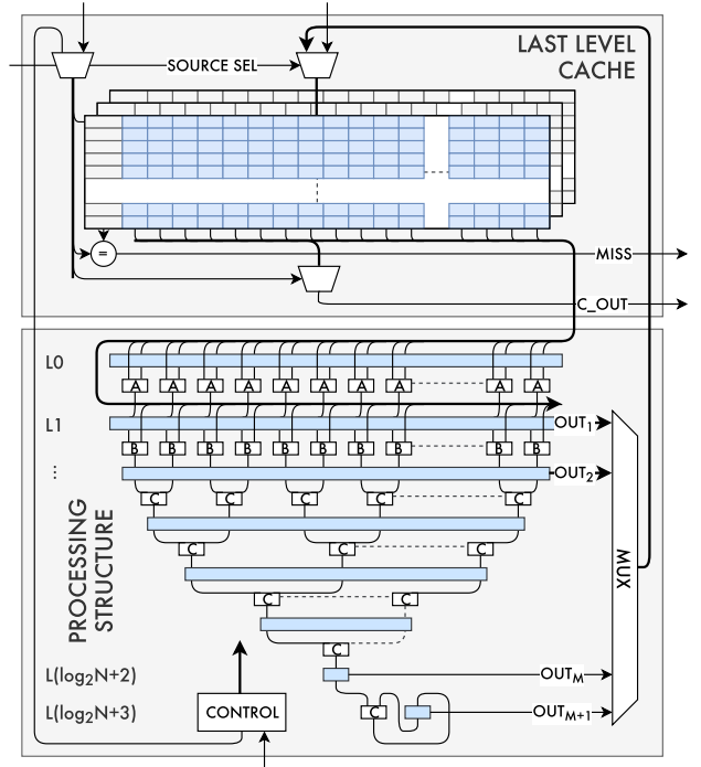
Fig. 4 Processing structure of the CCS.
