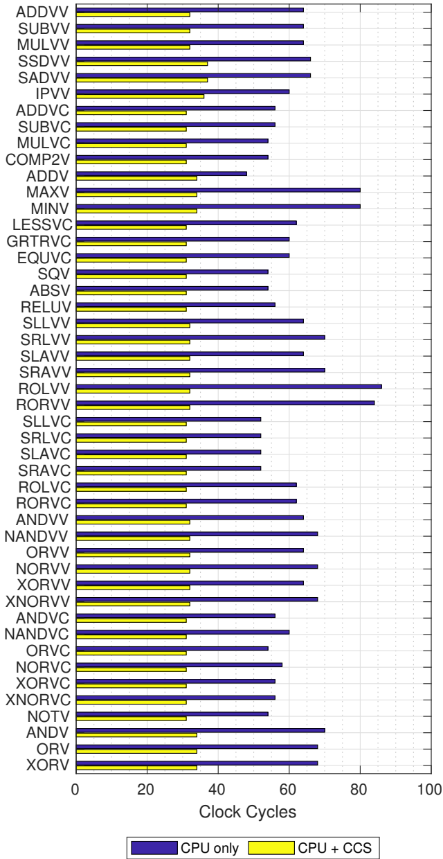
Fig. 6 Performance results of a set of microbenchmarks, each one corresponding to a CCS command, when executed using only the reference CPU or the CCS.
