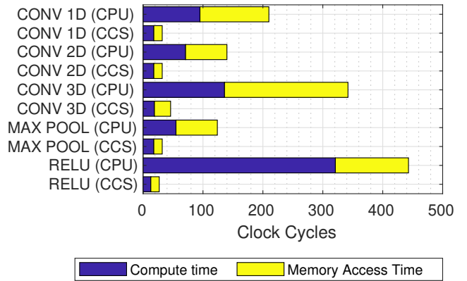
Fig. 8 Performance results regarding five kernels commonly used by CNNs, showing the time dedicated to accessing the memory and the actual computation time.
