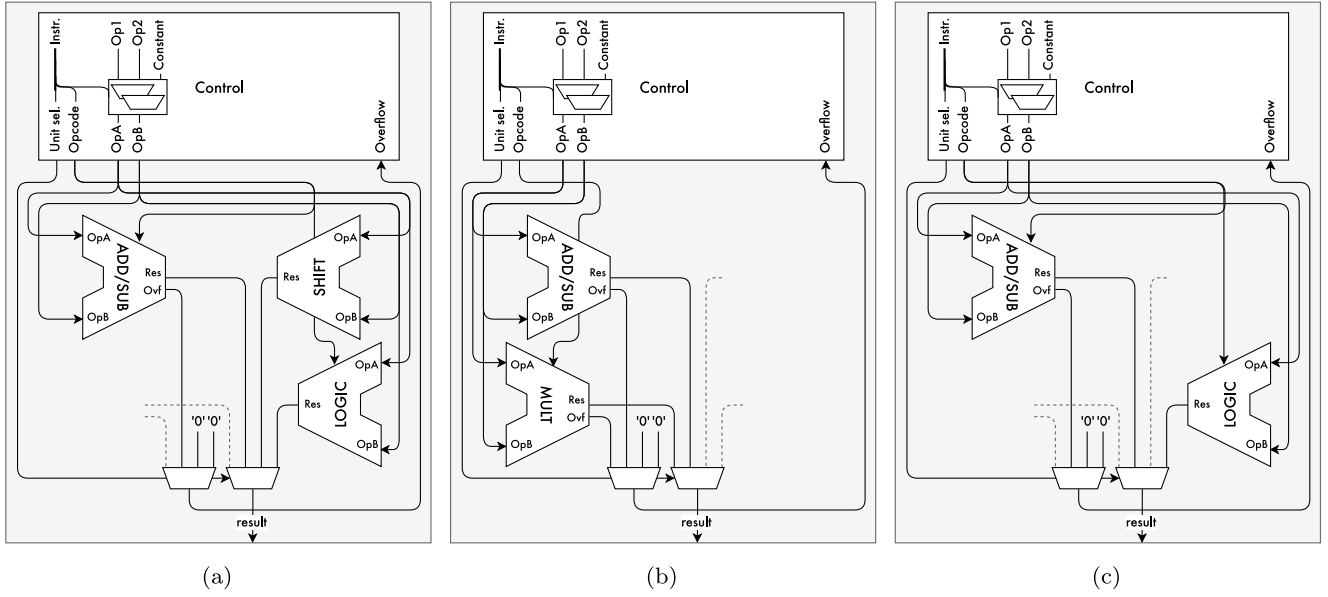
Fig. 5 FUs that compose the proposed CCS: (a) first level units, integrating an adder/subtractor, a shifter and a logical unit, (b) second level units containing an adder/subtractor and a multiplier, and (c) remaining FUs, including only an adder/subtractor and a logical unit.
