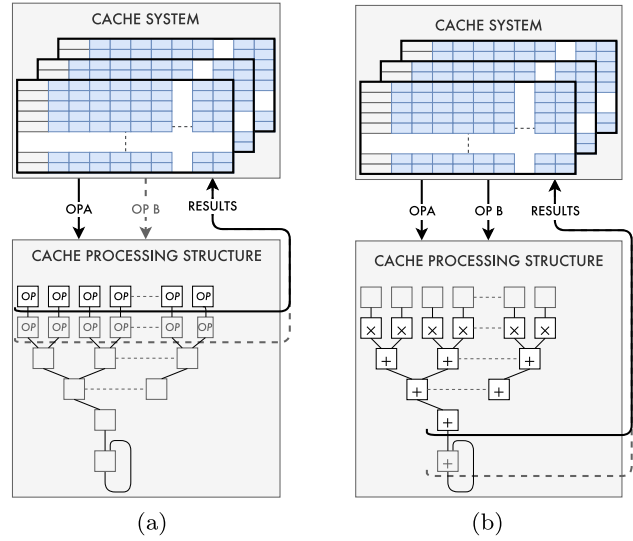
Fig. 3 Execution of two different instructions in the CCS: (a) ReLU; (b) dot-product.
