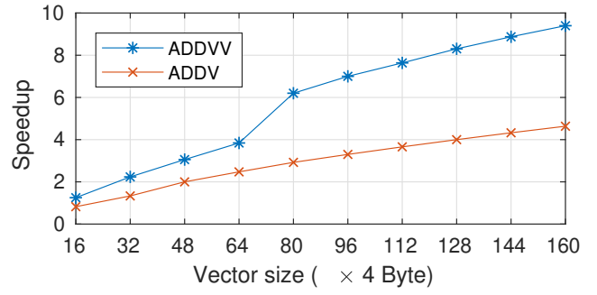
Fig. 7 Variation of performance gains with the size of the operands for a command of type map (ADDVV) and a command of type reduce (ADDV).
